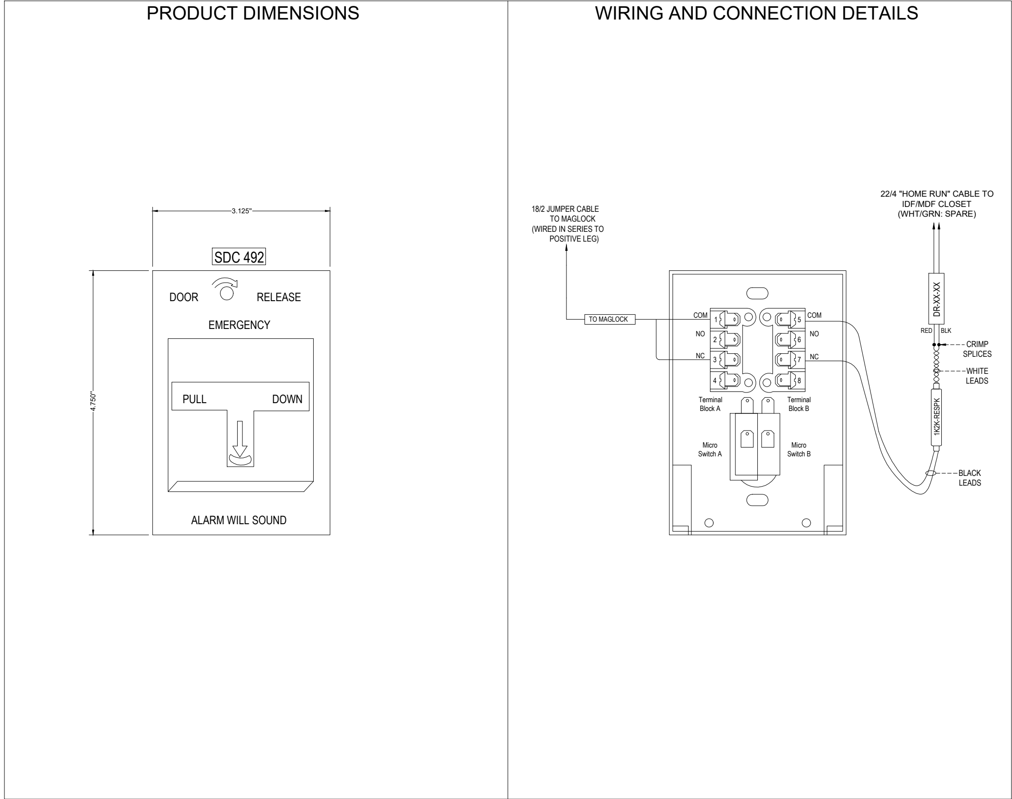
3 TYPICAL WALL-MOUNTED PULLSTATION DOOR RELEASE (DR-XX-XX)
