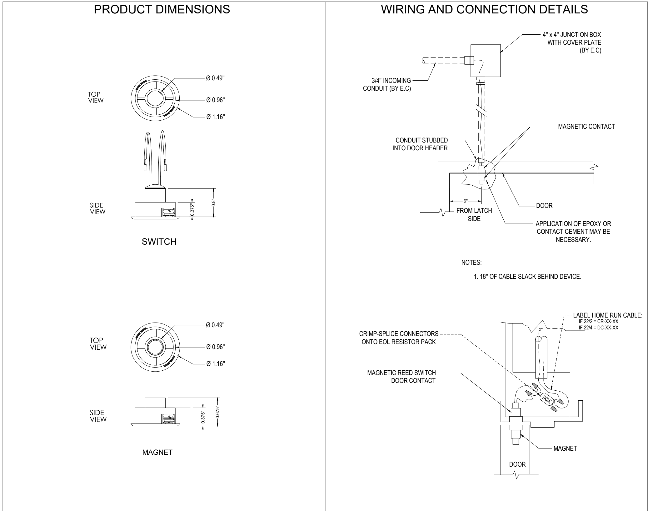
1 TYPICAL DOOR CONTACT(DC-XX-XX)
