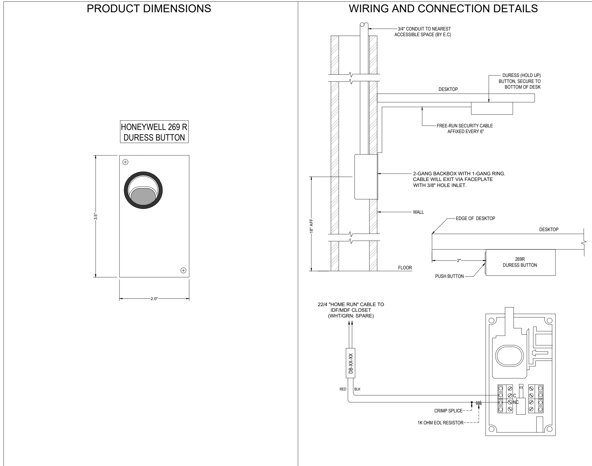
2 TYPICAL DURESS BUTTON (DB-XX-XX)
