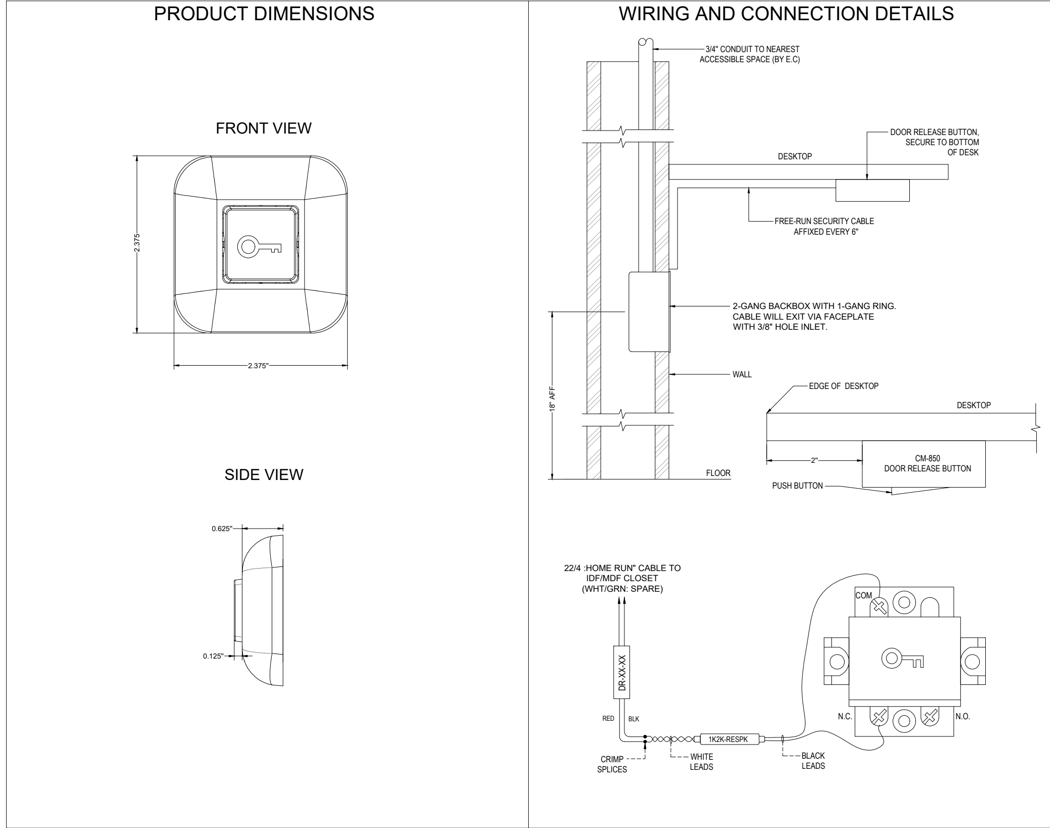
4 TYPICAL UNDER-DESK DOOR RELEASE (DR-XX-XX)
